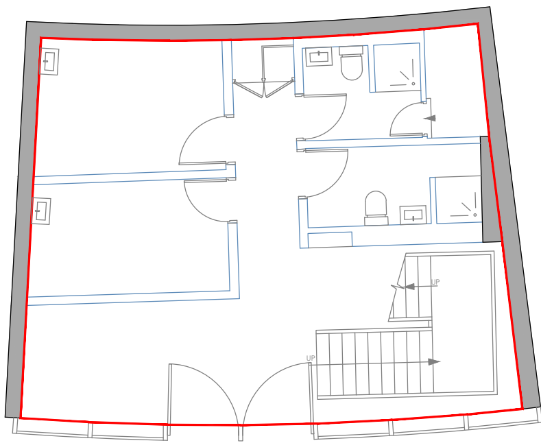
GROUND FLOOR HESTER ROAD
