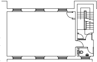
TYPICAL FLOOR PLAN (Not to scale)
